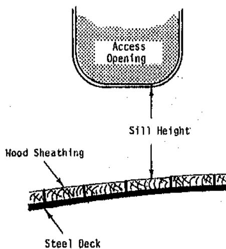
Minimum Sill Heights
