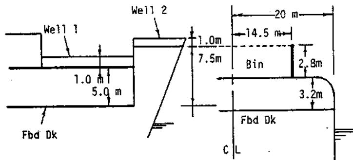
Figure 94. Freeing Ports-Adjustment Factors Above Freeboard Deck Level
