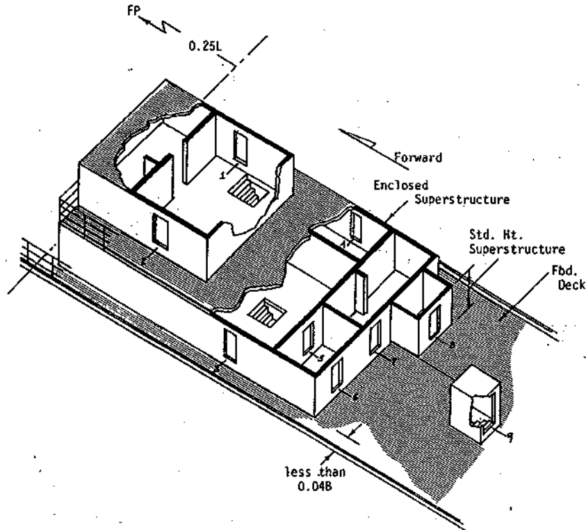
Minimum Sill Heights (Illustrated in Above Figure)
