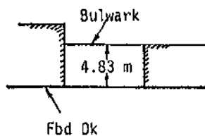
Figure 93. Freeing Ports- Adjustment Factors Freeboard Deck Level
